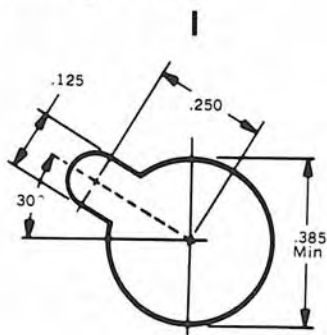
Four-Contact 126-214, 126-214-1001, 126-233, 126-215-1002 only
