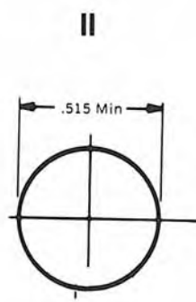
5-7-9 Contact Hex Nut Type Without Panel Locking Clip
